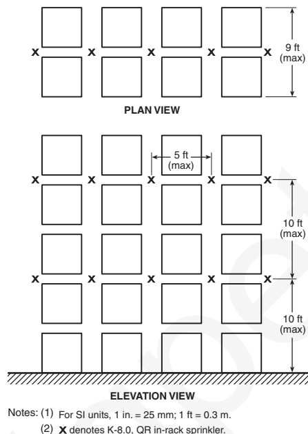
FIGURE 16.6.4(c) Double-Row Rack Sprinkler Layout 8 — Option #2.
