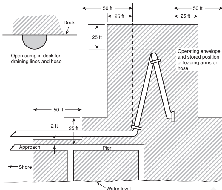
FIGURE 29.3.22 Area Classification for a Marine Terminal Handling Flammable Liquids.
