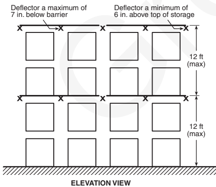
FIGURE 16.6.1.1(a) Single-Row Rack Sprinkler Layout for Design Scheme “A.”
