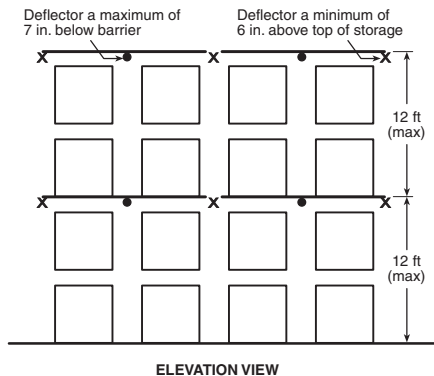
FIGURE 16.6.1.1(b) Double-Row Rack Sprinkler Layout for Design Scheme “A.”
